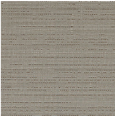
Fossil
